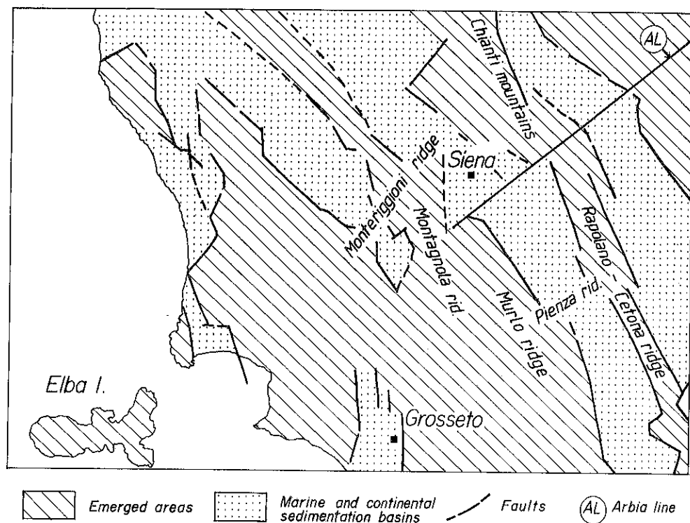
Fig. 1 - Distribution of the main neogenic sedimentation basins in Southern Tuscany.
