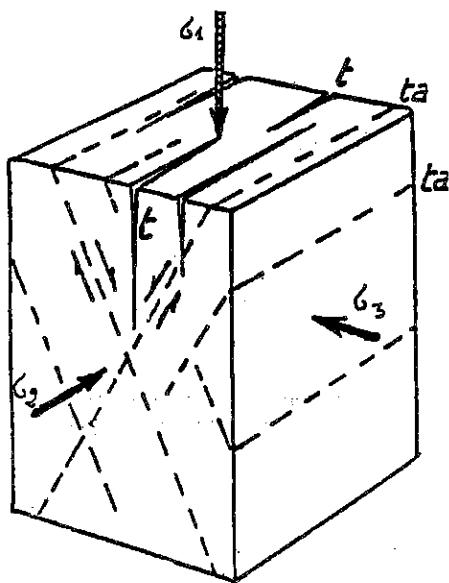
Fig. 7 - Orientation of shear fractures (ta) and tensional fractures (t) with respect to the main directions of pressure ( \sigma_1 - \sigma_2 - \sigma_3 ) (from Wilson 1961).
