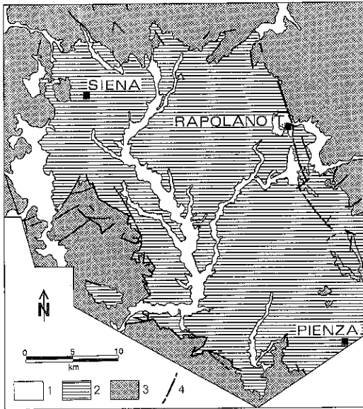
Fig. 2 - Geological sketch map of the Siena basin (from Costantini et al. 1982). 1. Quaternary deposits; 2. Sandy and argillaceous neogenic deposits; 3. Miocene and older; 4. Faults.
