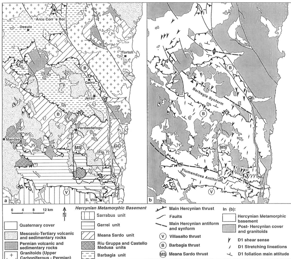
Fig. 2. (a) Tectonic map of the Hercynian basement of SE Sardinia, see Fig. 1 for location. (b) Structural map of the same area, showing D_1 stretching lineations and shear sense indicators in mylonites (from asymmetric porphyroclasts, shear bands, S-C fabrics, crystallographic preferred orientations, etc.). Arrows of shear sense indicators point to the transport direction of the hanging wall, irrespective of their plunge in the field.
