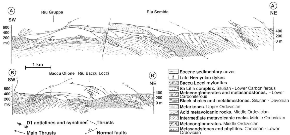
Fig. 8. Profiles in the Riu Grappa-Baccu Locci area. See Fig. 7 for profile traces.
