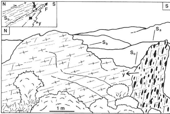
Fig. 6. Drawing after photograph of an outcrop in the Gerrei unit (North of Arcu'e Pesu, UTM coordinates 32SNJ38188168, see Fig. 7 for location) where the stratigraphic contact between Cambrian conglomerates ('Rio Ceraxa formation', on the right) and the younger metavolcanic rocks of the 'Porfiroidi formation' (on the left), is exposed. Normal limb of the D_1 Arcu'e Pesu anticline. Two foliations are present in this outcrop, both folded by D_2 and D_3 folds: a steeply dipping foliation ( S_a ), parallel to the stratigraphic contact ( S_0 ), cut by a spaced flat-lying crenulation cleavage ( S_b ). Field mapping has shown that S_b foliation is parallel to the Meana Sardo thrust and that the S_a foliation is the axial plane foliation ( S_1 ) of the large-scale isoclinal D_1 folds in the Gerrei unit. S_b foliation is therefore thrust-related and developed during early stages of D_1 crustal thickening.
