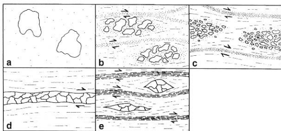
Fig. 10. Evolution of microstructures in the Baccu Locci mylonites. Strain and recrystallization increase from (a) to (e). (a) Undeformed acid volcanic rocks with large quartz crystals in a fine grained quartz-rich matrix. (b) Strain and plastic deformation occurred in narrow quartz layers in the matrix, and porphyroclasts are only locally recrystallized. (c) Porphyroclasts are now fully recrystallized, but strain still localized in the matrix. (d) Coalescence of totally recrystallized porphyroclasts led to quartz-rich layers, that then accommodated most of strain. (e) Increasing mica content due to feldspar breakdown led to viscous flow localization in phyllosilicate-rich levels and to boudinage of dynamically recrystallized quartz ribbons.
